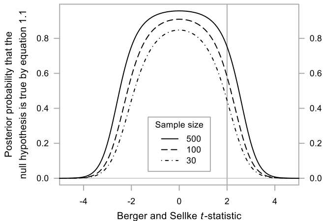
Figure R.1. The relationship between the Berger and Sellke t -statistic and the posterior probability that the null hypothesis is true for three different sample sizes assuming that the prior probabilities that the research and null hypotheses are true are both 0.5. The figure was generated using Berger and Sellke's equation 1.1 for computing the posterior probability from the t -statistic. Macnaughton (2021) gives the R program used to generate the figure.
