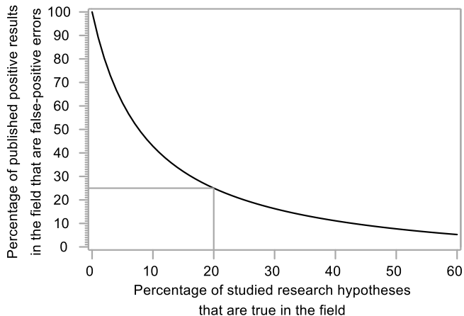
Figure H.1. The percentage of published positive results that are false-positive errors in a field of empirical research as a function of the percentage of studied research hypotheses that are true in the field under the assumptions discussed in the text. The vertical and horizontal gray lines illustrate the example discussed in the text. The graph is based on ideas introduced by Jager and Leek (2014).
