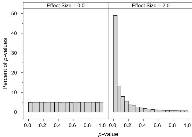
Figure D.1. Two histograms, each showing the distribution of the p -values that we will obtain if we repeat a particular research study over and over, each time collecting fresh data. Each histogram was obtained through a computer simulation. The computer programs to generate this figure are at tas-nejm.com
