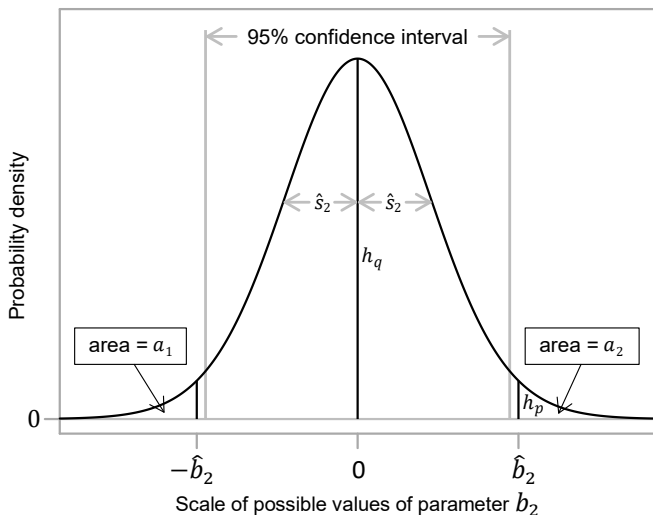
Figure C.1. A graph showing the estimated sampling distribution (estimated probability density function) of the estimated value of parameter b_2 of a linear regression model equation if the relevant null hypothesis is true. The value \hat{b}_2 is shown twice on the horizontal axis and the value \hat{s}_2 is shown twice partway up the graph.
